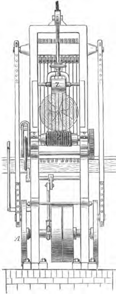
Fig. 300.—Multiple saw.
